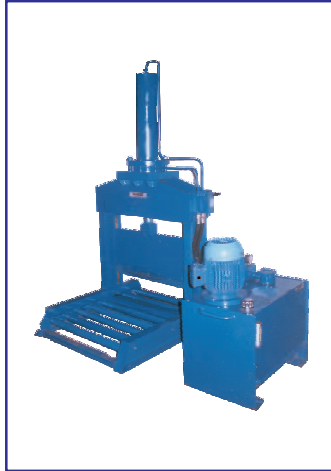
30 T hydraulic press for rubber bail cutting
